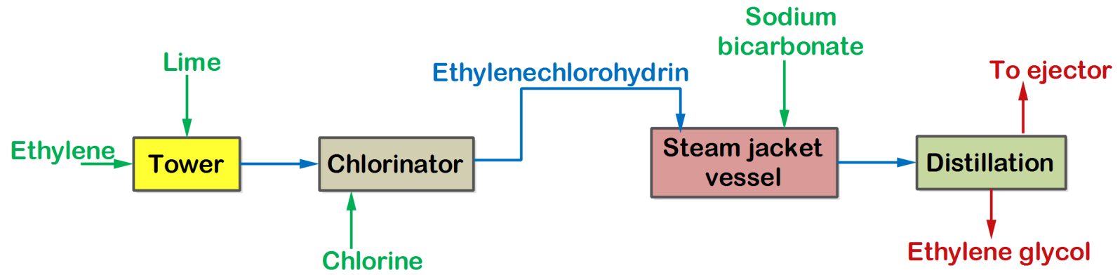
Figure: Manufacture of Ethylene glycol via ethylenechlorohydrin
